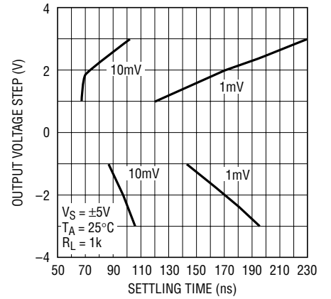
Output Voltage Step vs Settling Time, A_V = 1
