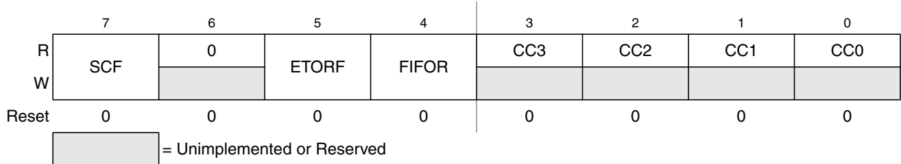
Figure 16-9. ATD Status Register 0 (ATDSTAT0)
