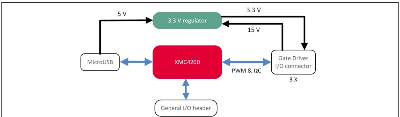
Figure 2 Eval-1ED38x0DCT block diagram
