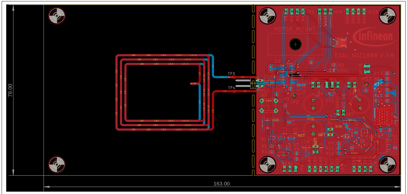
Figure 4 Layout, top view
