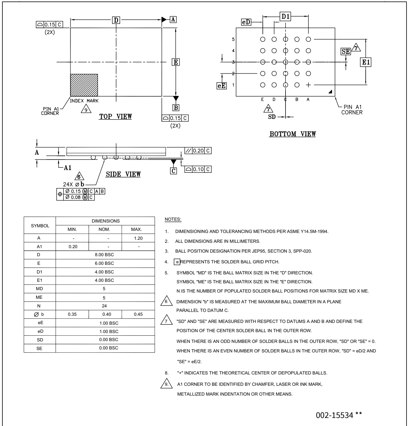
Figure 154 24-ball FBGA (8 × 6 × 1.2 mm) package outline, 002-15534
