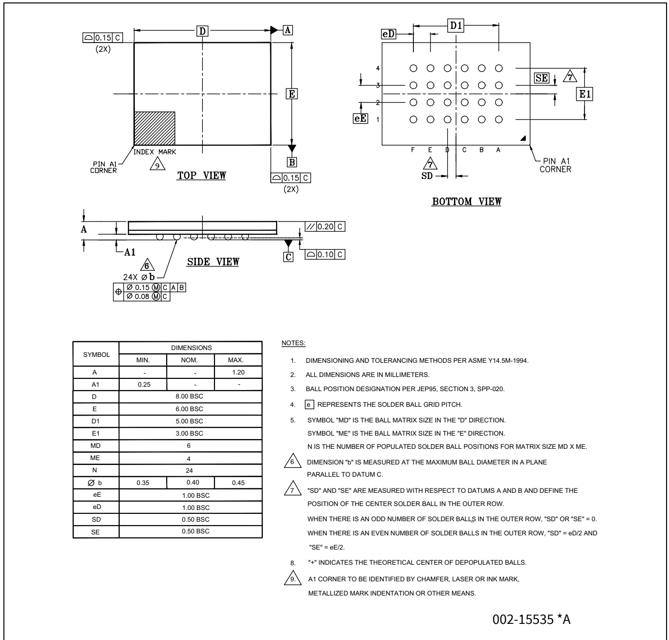
Figure 155 24-ball FBGA (8 × 6 × 1.2 mm) package outline, 002-15535
