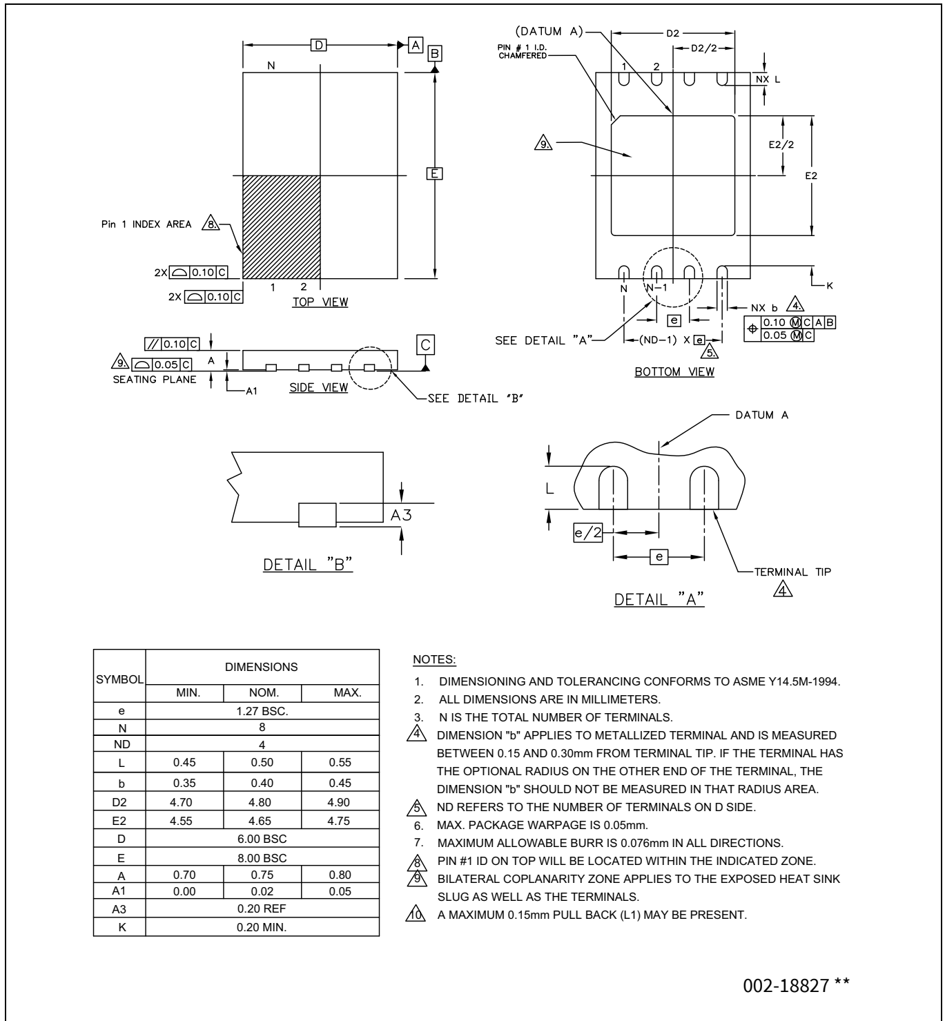
Figure 153 8-lead DFN ((6 × 8 × 0.8 mm) 4.80 × 4.65 mm E-Pad (Sawn)) package outline, 002-18827
