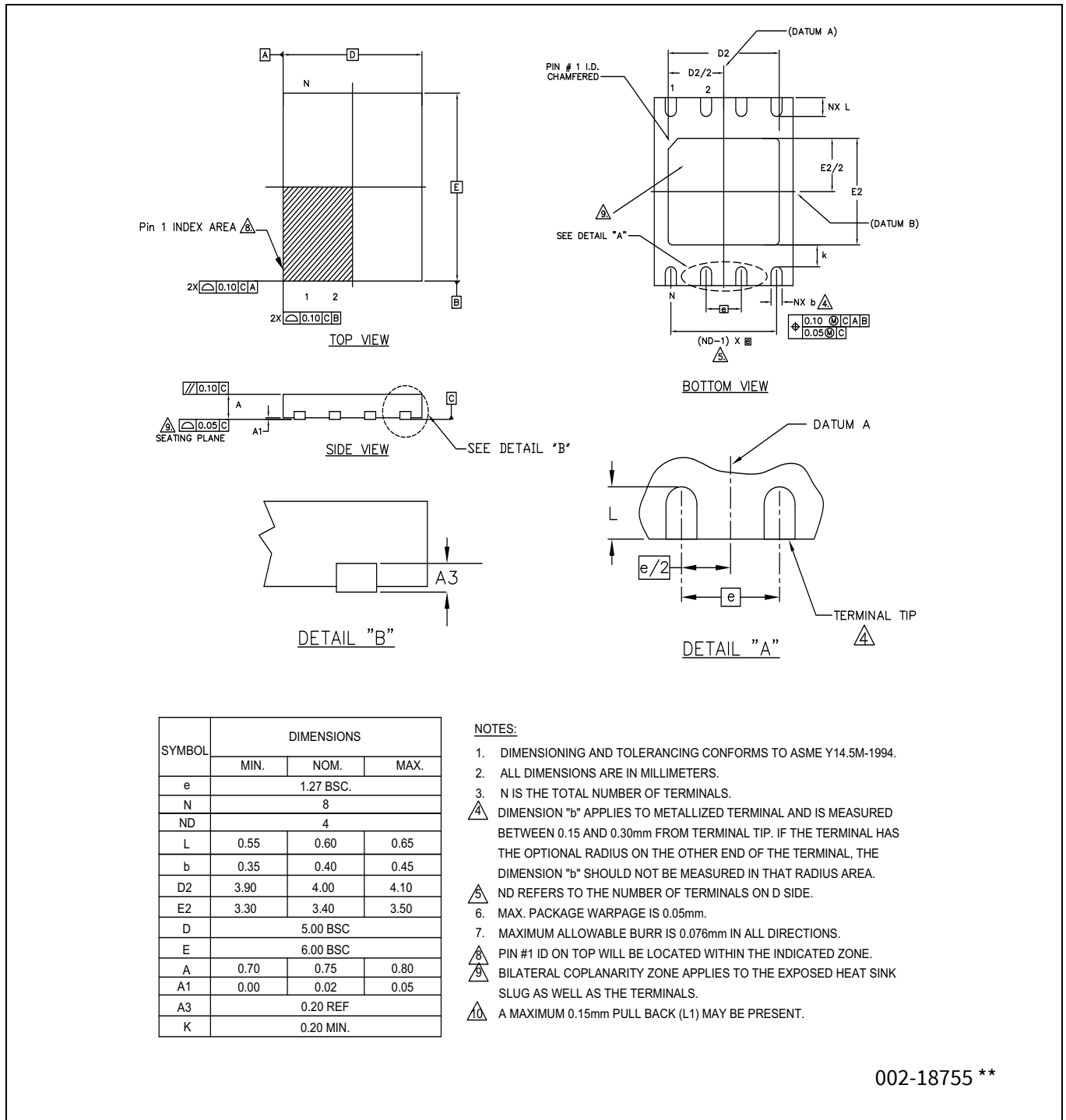
Figure 152 8-lead DFN ((5 × 6 × 0.8 mm) 4.0 × 3.4 mm E-Pad (Sawn)) package outline, 002-18755
