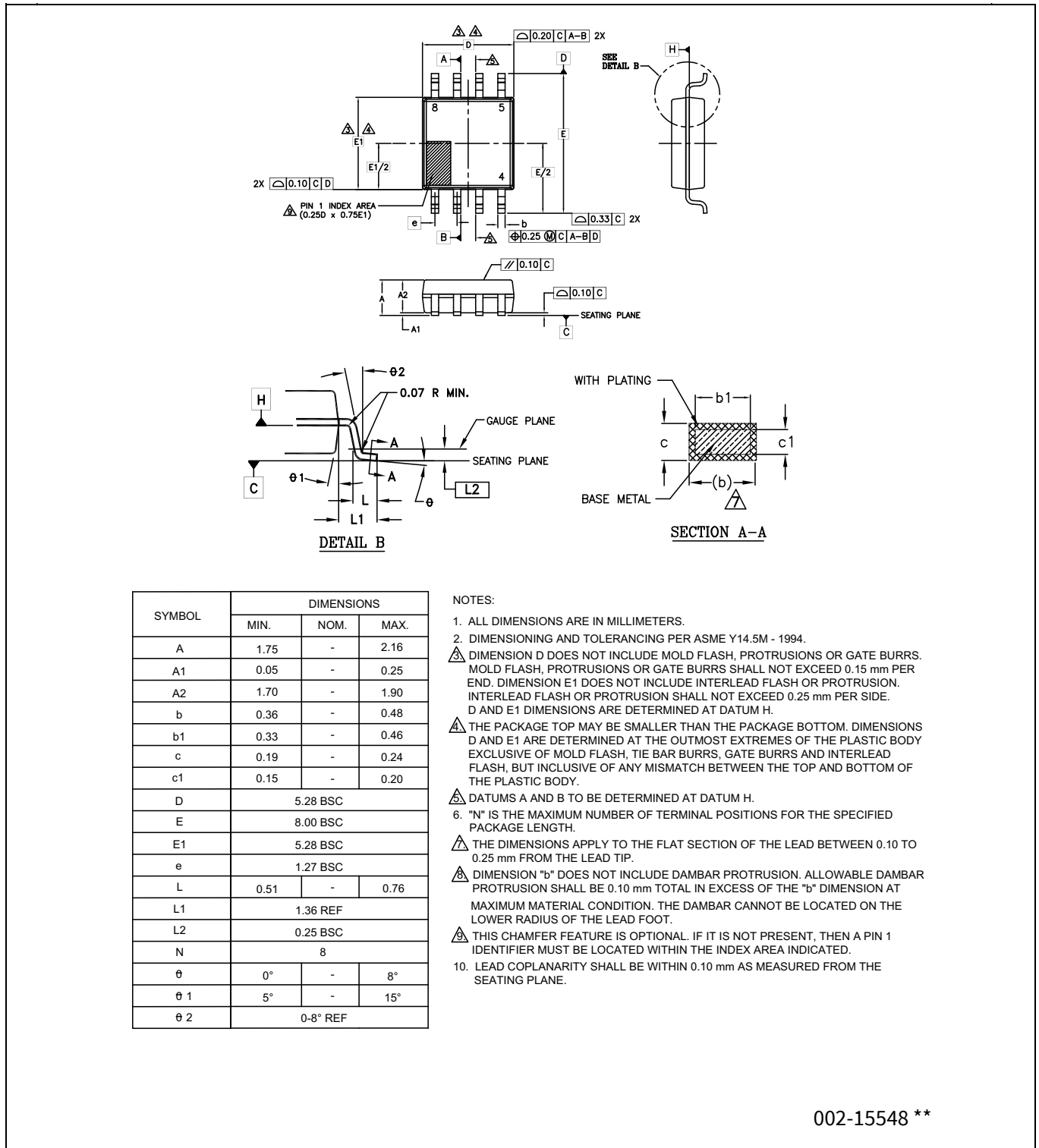
Figure 151 8-lead SOIC (5.28 x 5.28 x 2.16 mm) package outline, 002-15548
