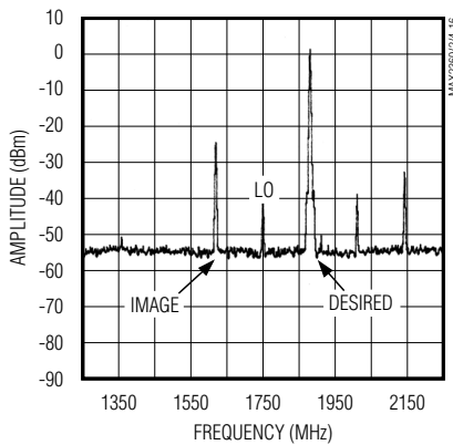
RFHO OUTPUT SPECTRUM
