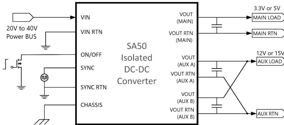
Figure 3-3. SA50-28T AUX Split Outputs Application Circuit
