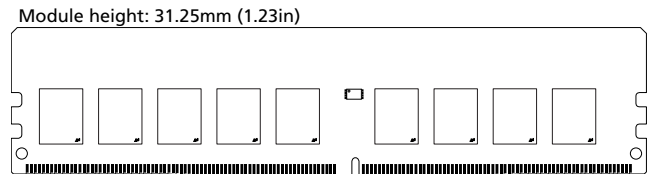
Figure 1: 288-Pin UDIMM (R/C-E1)
