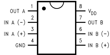
SOP & MSOP Package
