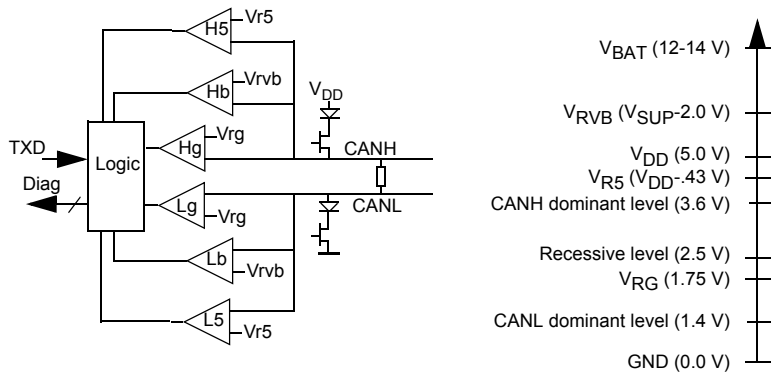
Figure 38. CAN Bus Simplified Structure Truth Table for Failure Detection
