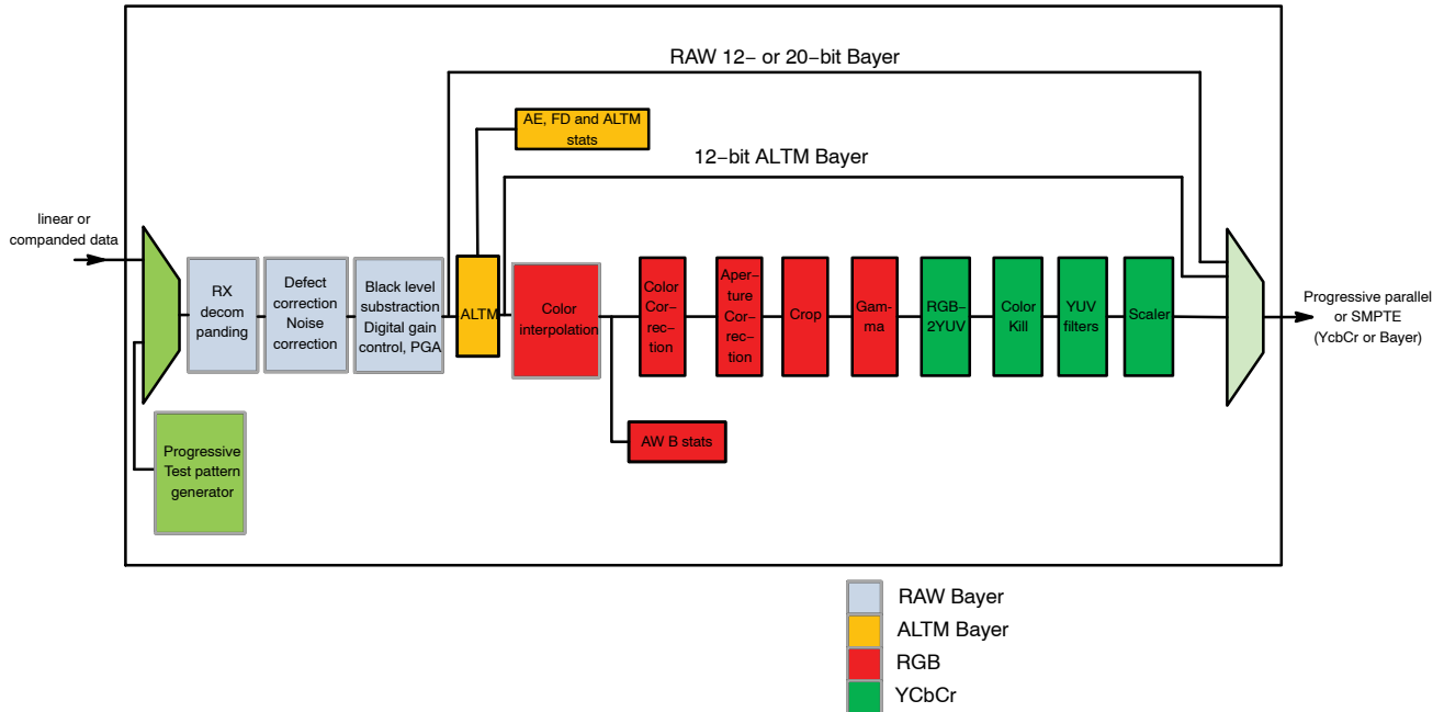
Figure 9. Continuous Mode
