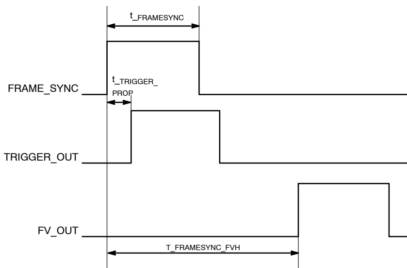
Figure 7. Single-Shot Mode
