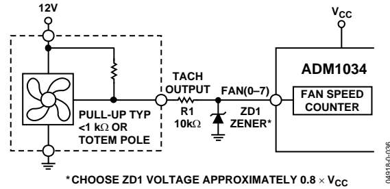
Figure 38. Fan with Strong TACH. Pull-Up to >V_{CC} or Totem-Pole Output, Clamped with Zener and Resistor.
