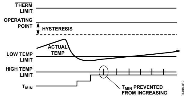
Figure 75. T_{\text{MIN}} Adjustments Limited by the High Temperature Limit
