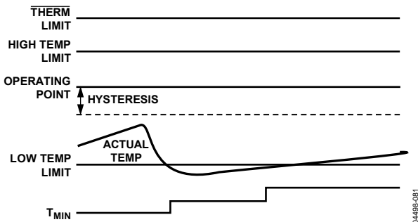
Figure 74. Increasing T_{\text{MIN}} for Quiet Operation
