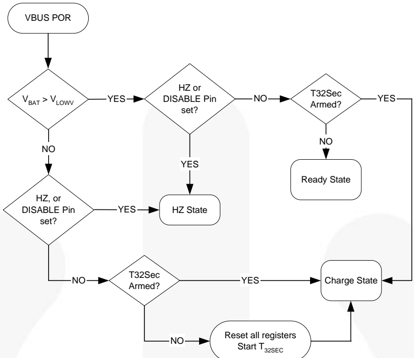
Figure 38. Charger V BUS POR Flow Chart
