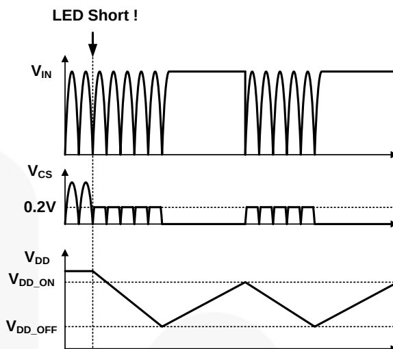
Figure 20. Waveforms at Short-LED Condition
