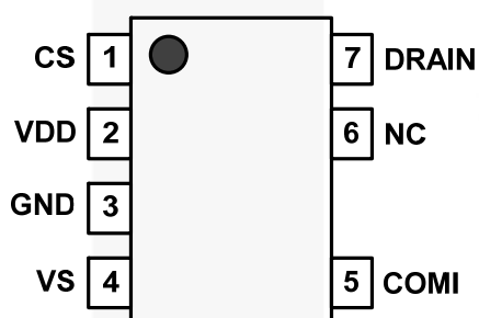
Figure 4. Pin Configuration
