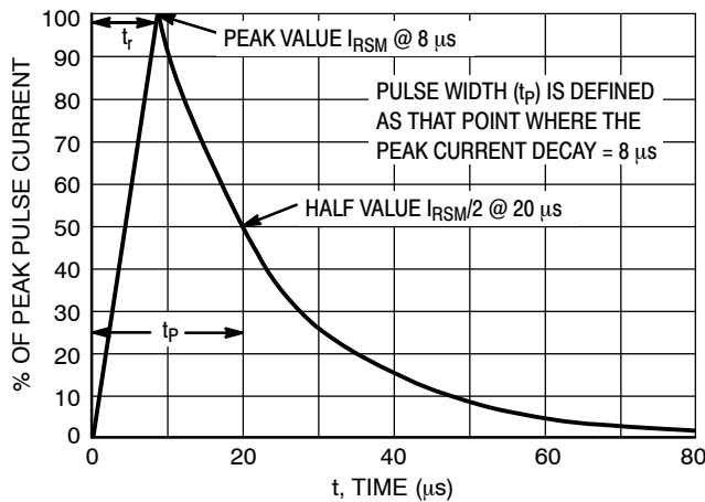
Figure 15. 8 x 20 μs Pulse Waveform
