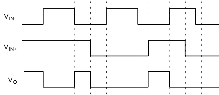
Figure 54. Input/Output Relationship
