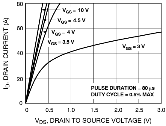
Figure 13. On-Region Characteristics
