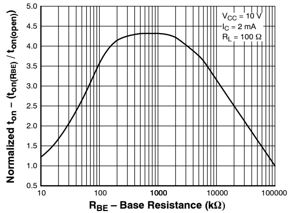
Figure 8. Normalized t_{\text{on}} vs. R_{\text{BE}}
