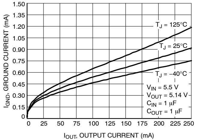
Figure 16. Ground Current vs. Load Current - V OUT = 5.14 V
