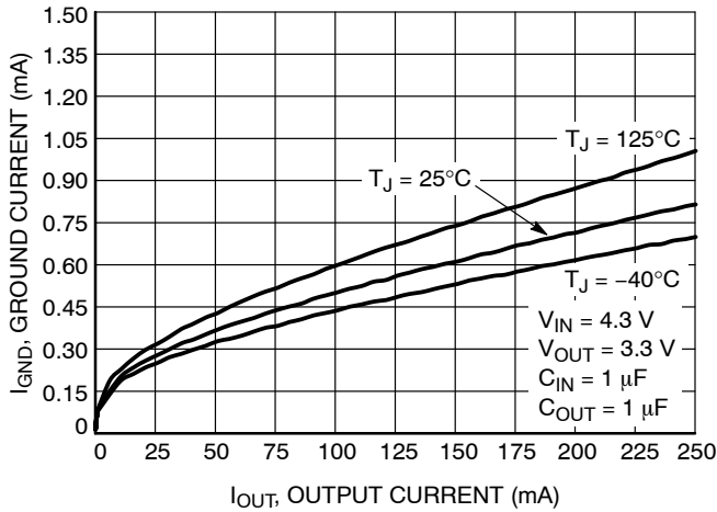
Figure 15. Ground Current vs. Load Current - V OUT = 3.3 V
