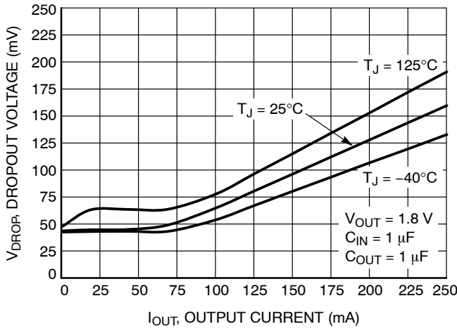
Figure 17. Dropout Voltage vs. Load Current - V OUT = 1.8 V
