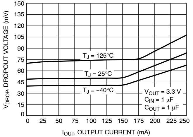
Figure 18. Dropout Voltage vs. Load Current - V OUT = 3.3 V
