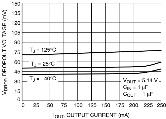
Figure 19. Dropout Voltage vs. Load Current - V OUT = 5.14 V
