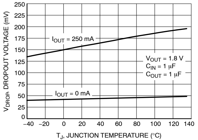
Figure 20. Dropout Voltage vs. Temperature - V OUT = 1.8 V
