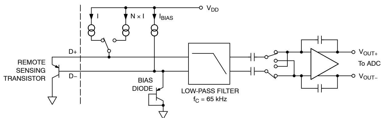
Figure 18. Signal Conditioning
