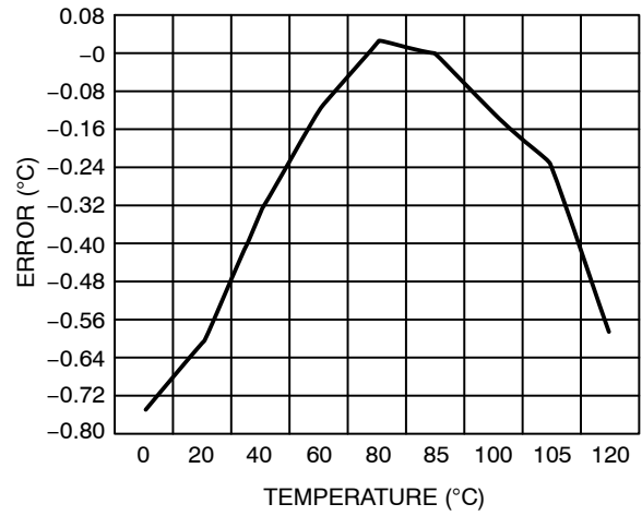
Figure 10. Remote Sensor Error
