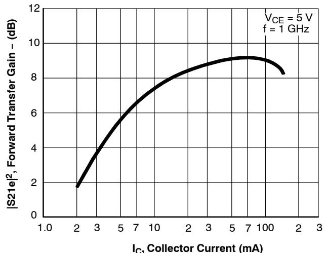
Figure 6. |S_{21e}|^2 - I_C
