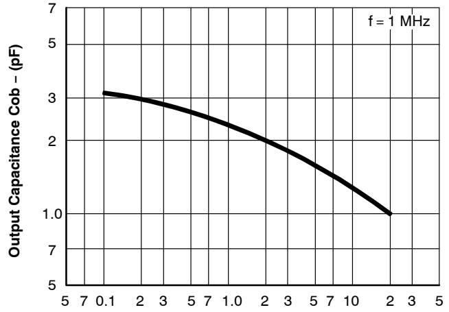
Figure 4. C_{ob} - V_{CB}
