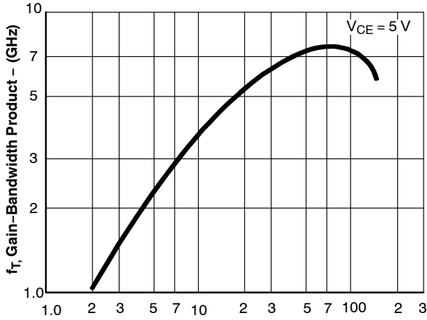
Figure 3. f_T - I_C
