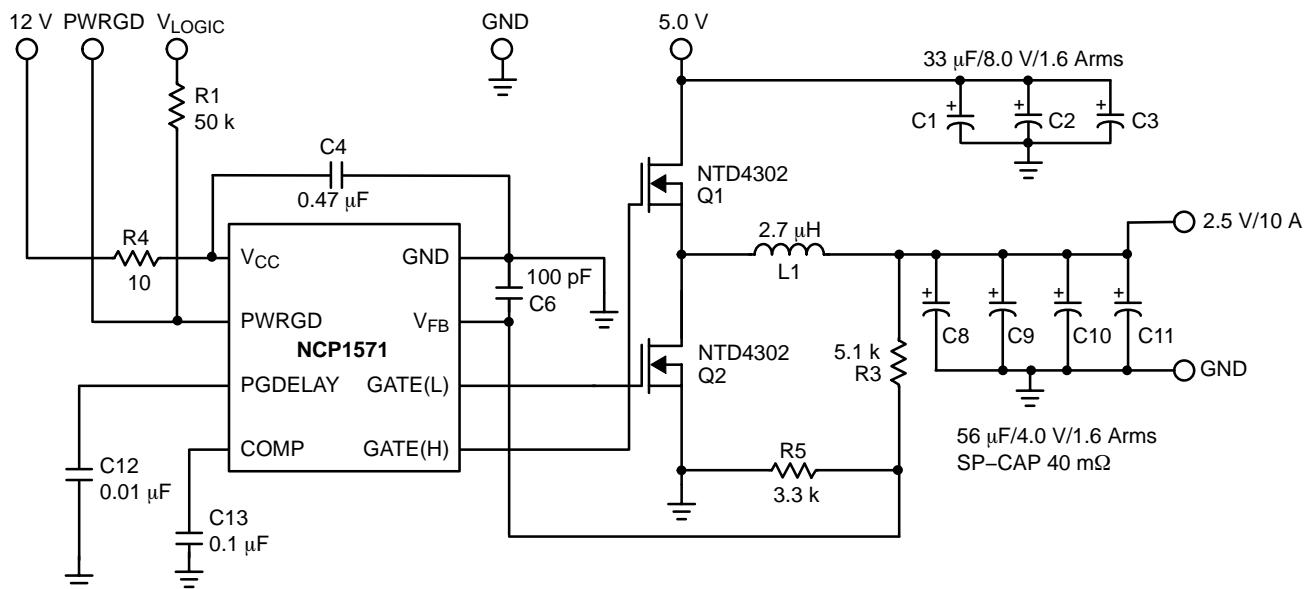
Figure 1. Applications Circuit
