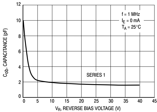
Figure 24. Output Capacitance
