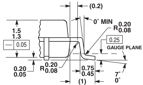
VIEW AA
