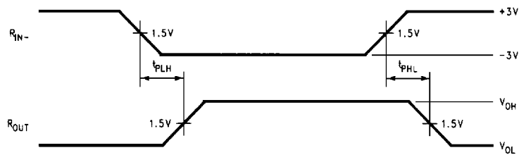
FIGURE 5. Receiver Propagation Delay Waveform
