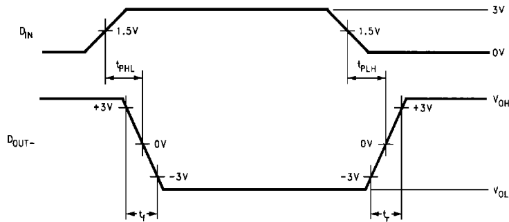
FIGURE 3. Driver Propagation Delay and Transition Time Waveform
