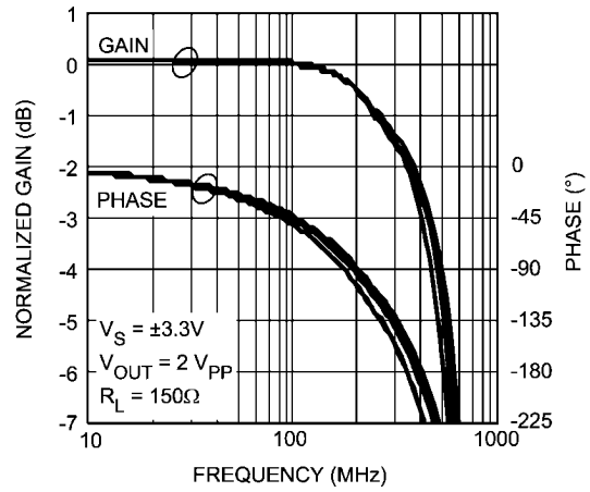
2 V PP Frequency Response
