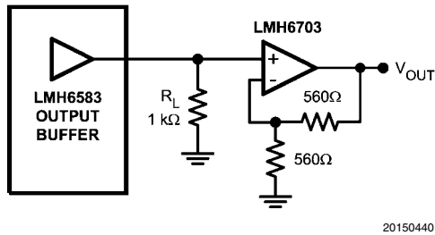
FIGURE 6. Buffered Output
