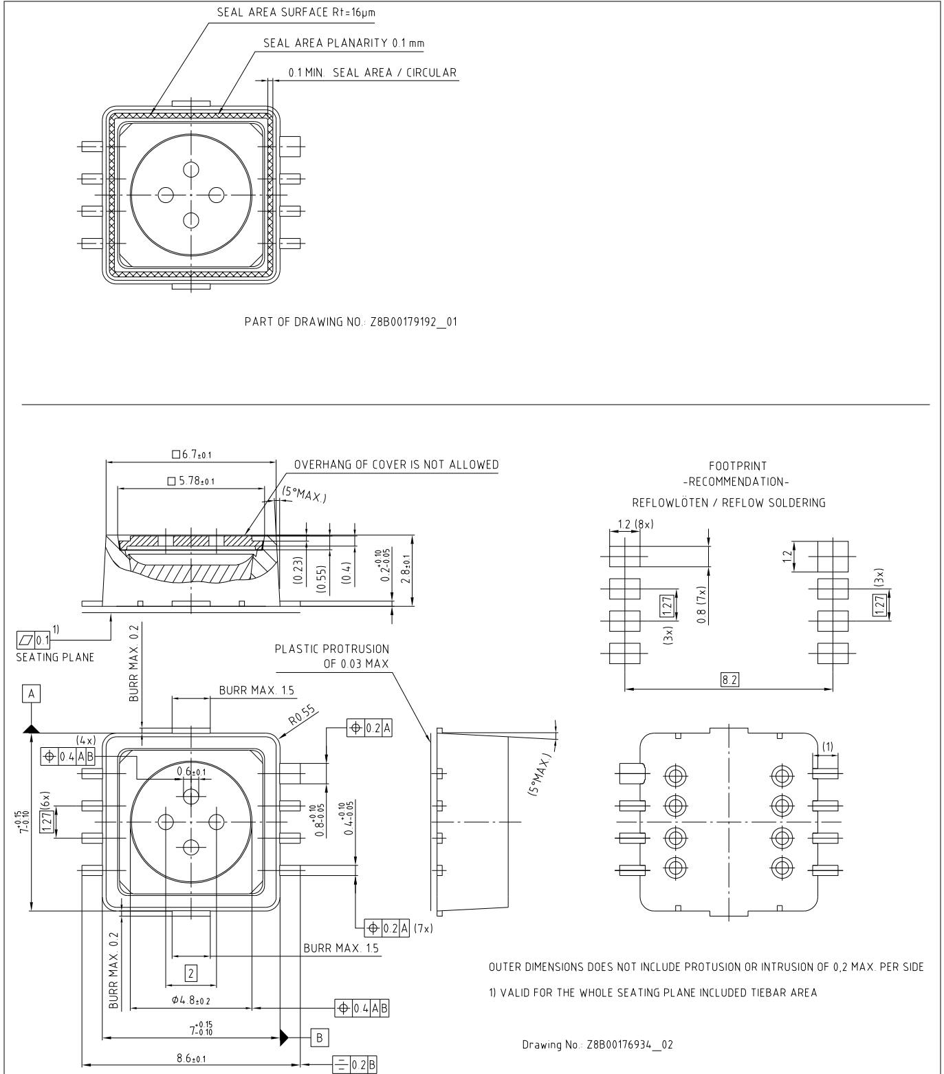
Figure 2 PG-DSOF-8-164 package outline (all dimensions in mm)
