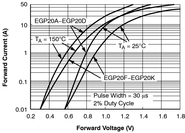
Figure 3. Forward Characteristics
