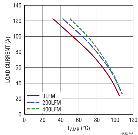
Figure 46. 12V IN to 0.7V OUT Derating Curve, No Heat Sink
