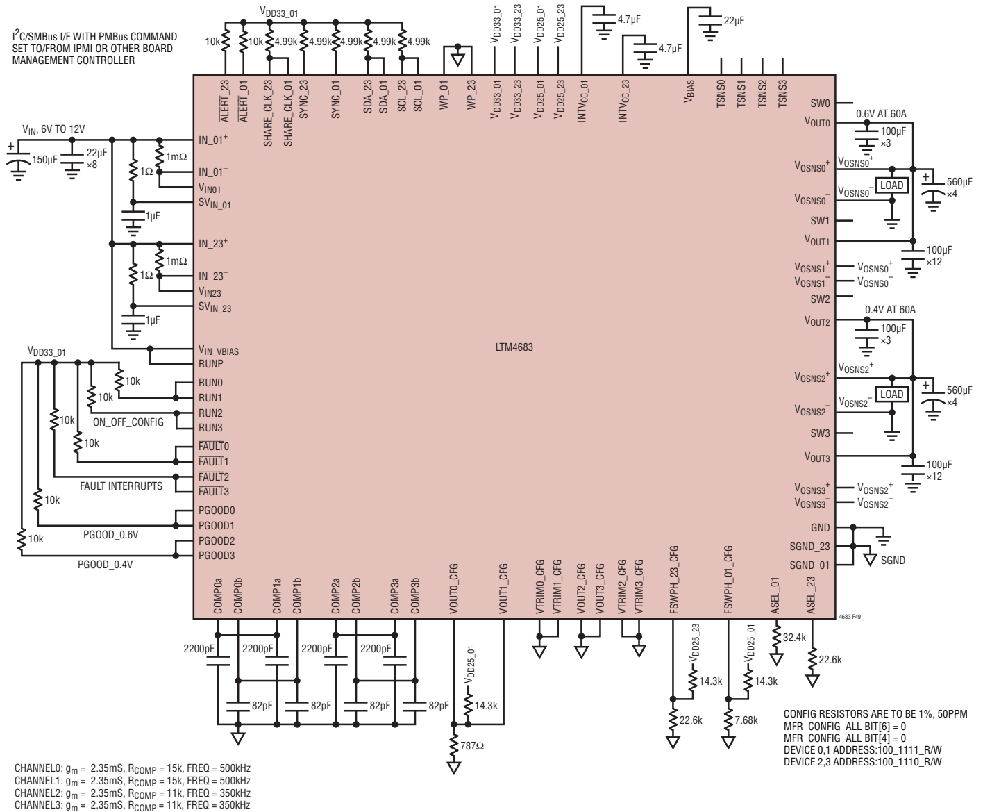
Figure 49. 0.6V and 0.4V Outputs at 60A with Providing I 2 C/SMBus/PMBus Serial Interface
