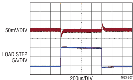
FIGURE 48 CIRCUIT, 12V TO 0.6V, FREQ = 500kHz C_{\text{OUT}} = 560\mu\text{F} \times 4 POSCAP, 100\mu\text{F} \times 4 CERAMIC R_{\text{COMP}} = 13\text{k} , E\text{A-}g_m = 3.02\text{mS} , \text{COMP}/r_a = 4.7\text{nF} , \text{COMP}/r_b = 150\text{pF} I_{\text{OUT}} \text{ RANGE HIGH} , V_{\text{OUT}} \text{ RANGE LOW}
