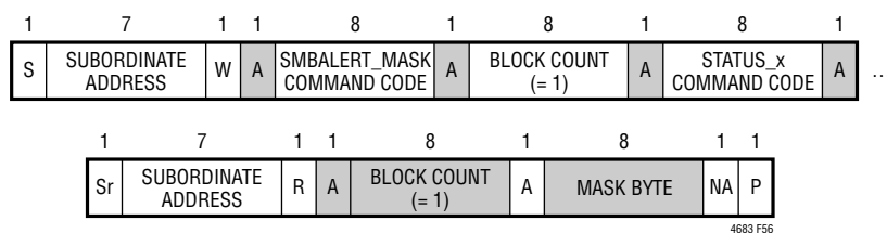
Figure 56. Example of Reading SMBALERT_MASK
