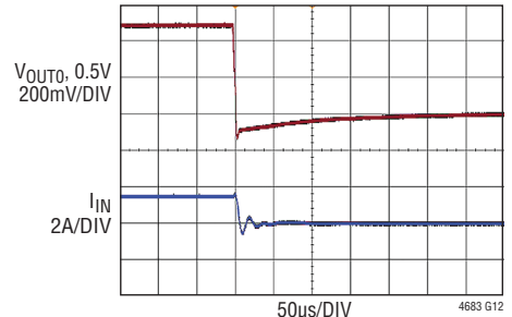
FIGURE 48 CIRCUIT, 12V_{IN} , 31.25A LOAD ON V_{OUT0} PRIOR TO APPLICATION OF SHORT-CIRCUIT USE HIGH RANGE OF I_{OUT} SYSTEM SHORT-CIRCUIT USING LOW IMPEDANCE COPPER ACROSS OUTPUT (HARD SHORT)
