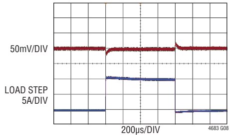
FIGURE 48 CIRCUIT, 12V TO 0.7V, FREQ = 575kHz C_{\text{OUT}} = 560\mu\text{F} \times 4 POSCAP, 100\mu\text{F} \times 4 CERAMIC R_{\text{COMP}} = 13\text{k} , E\text{A-}g_m = 3.02\text{mS} , \text{COMP}/r_a = 4.7\text{nF} , \text{COMP}/r_b = 150\text{pF} I_{\text{OUT}} \text{ RANGE HIGH} , V_{\text{OUT}} \text{ RANGE LOW}
