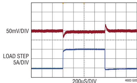
FIGURE 48 CIRCUIT, 12V TO 0.3V, FREQ = 250kHz C_{\text{OUT}} = 560\mu\text{F} \times 4 POSCAP, 100\mu\text{F} \times 4 CERAMIC R_{\text{COMP}} = 13\text{k} , E\text{A-}g_m = 3.02\text{mS} , \text{COMP}/r_a = 4.7\text{nF} , \text{COMP}/r_b = 150\text{pF} I_{\text{OUT}} \text{ RANGE HIGH} , V_{\text{OUT}} \text{ RANGE LOW}
