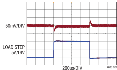
FIGURE 48 CIRCUIT, 12V TO 0.4V, FREQ = 350kHz C_{\text{OUT}} = 560\mu\text{F} \times 4 POSCAP, 100\mu\text{F} \times 4 CERAMIC R_{\text{COMP}} = 13\text{k} , E\text{A-}g_m = 3.02\text{mS} , \text{COMP}/r_a = 4.7\text{nF} , \text{COMP}/r_b = 150\text{pF} I_{\text{OUT}} \text{ RANGE HIGH} , V_{\text{OUT}} \text{ RANGE LOW}
