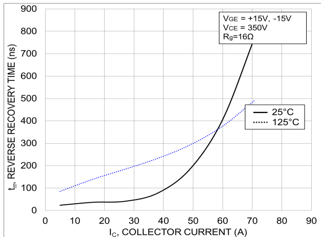
Figure 50. Typical Reverse Recovery Time vs. I_C
