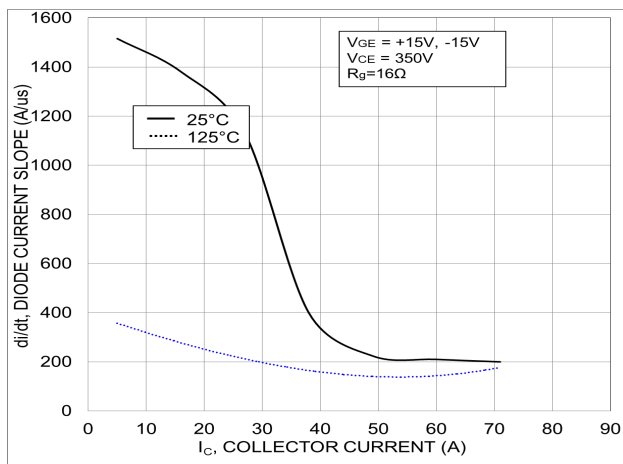
Figure 53. Typical di/dt Current Slope vs. I_C
