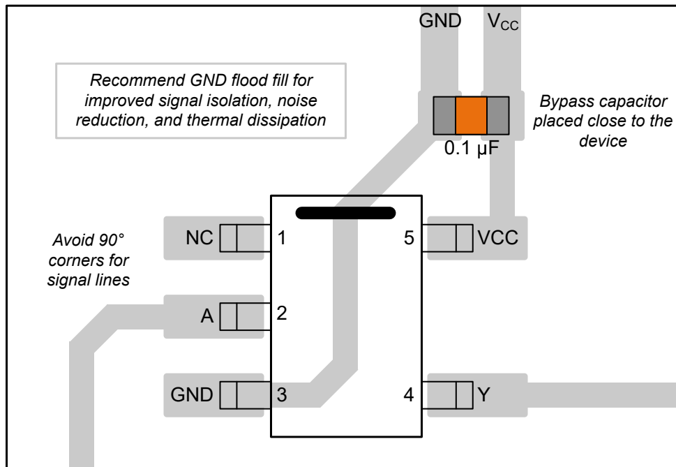
Figure 9-3. Example Layout for the SN74AHCT1G14-Q1
