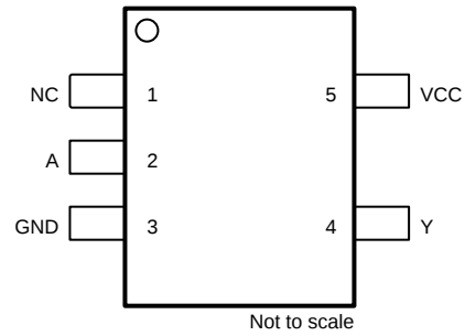
Figure 5-1. SN74AHCT1G14-Q1 DCK Package, 5-Pin SC-70 (Top View)
