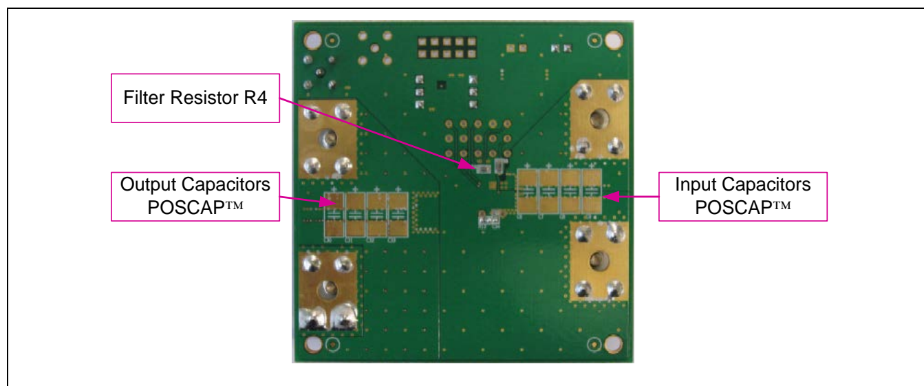
Figure 2.1 Bottom View of the ZSPM8010-KIT Open-Loop Evaluation Board Showing Capacitor Footprints
