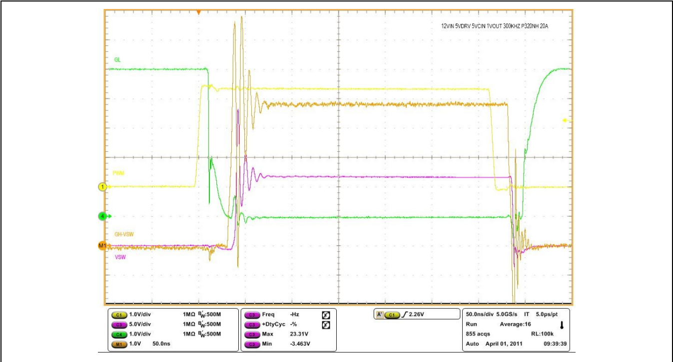
Figure 4.3 Switching Waveform
